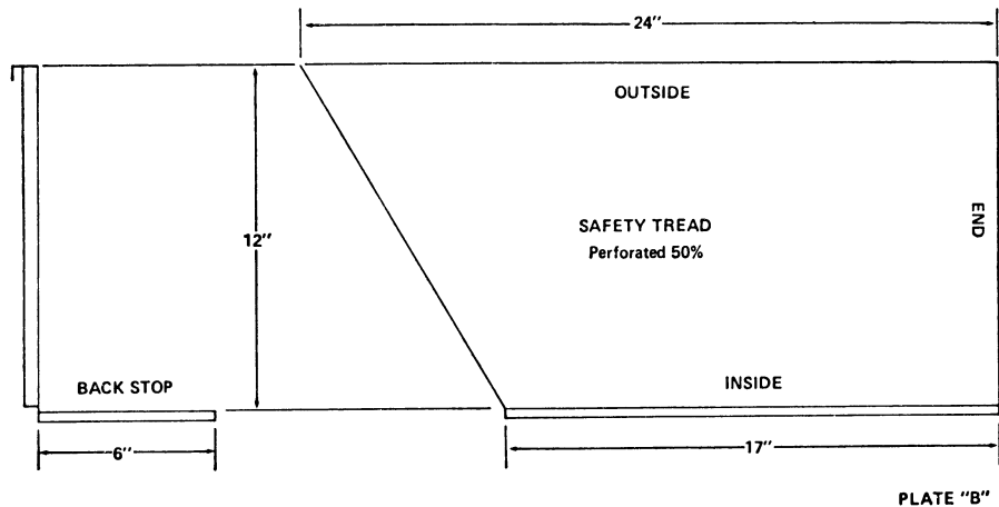
SWITCHING STEP SHOWING INSIDE RELIEF FOR CLEARANCE OF SIX-WHEEL TRUCK
